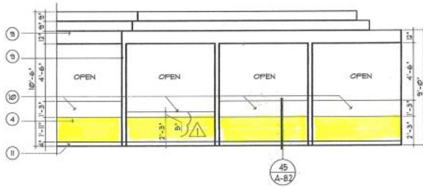
1 COUNTER ELEVATION (PUBLIC SIDE) 1/4" = 1'-0"
